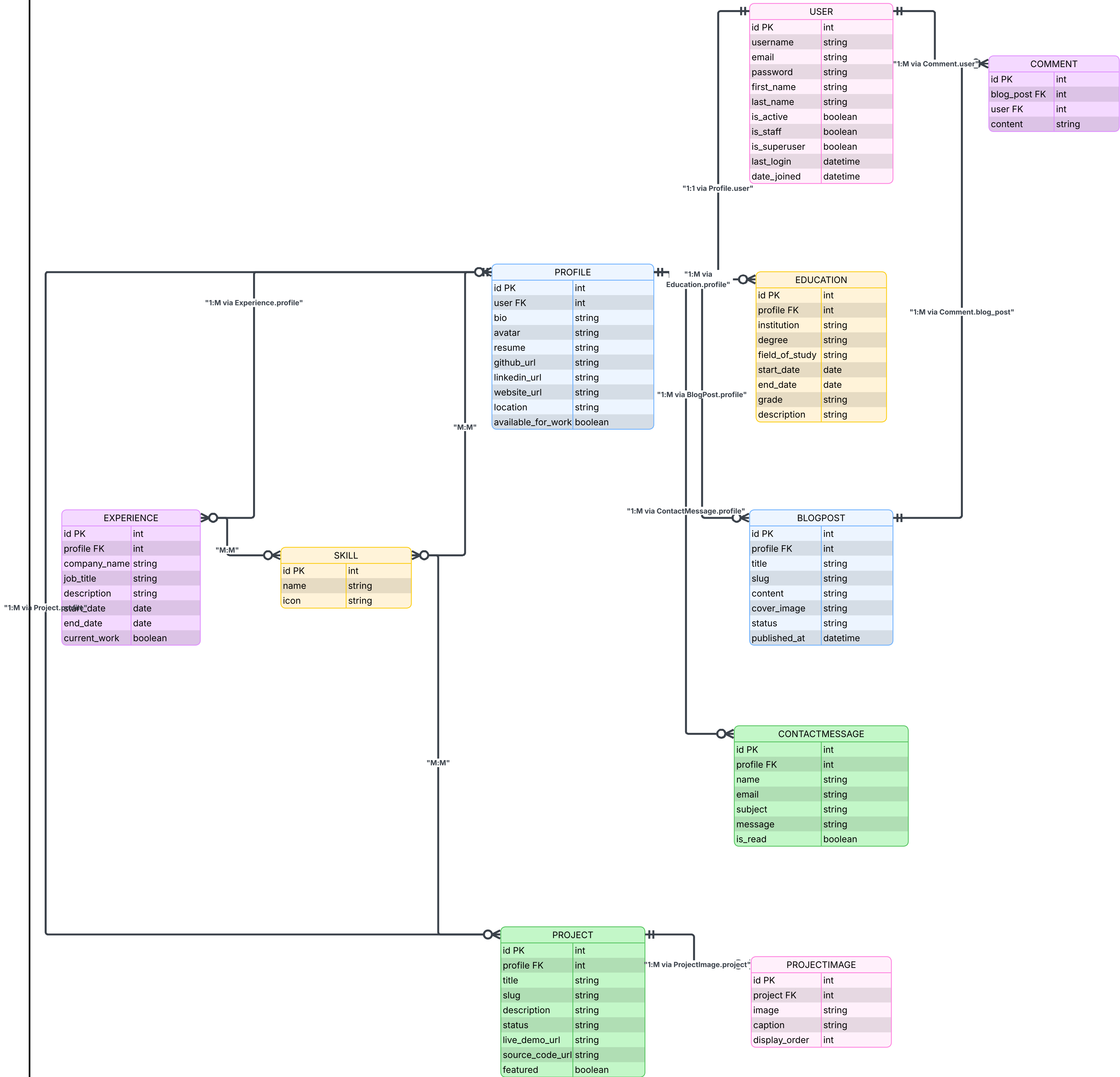
User & Profile ERD
